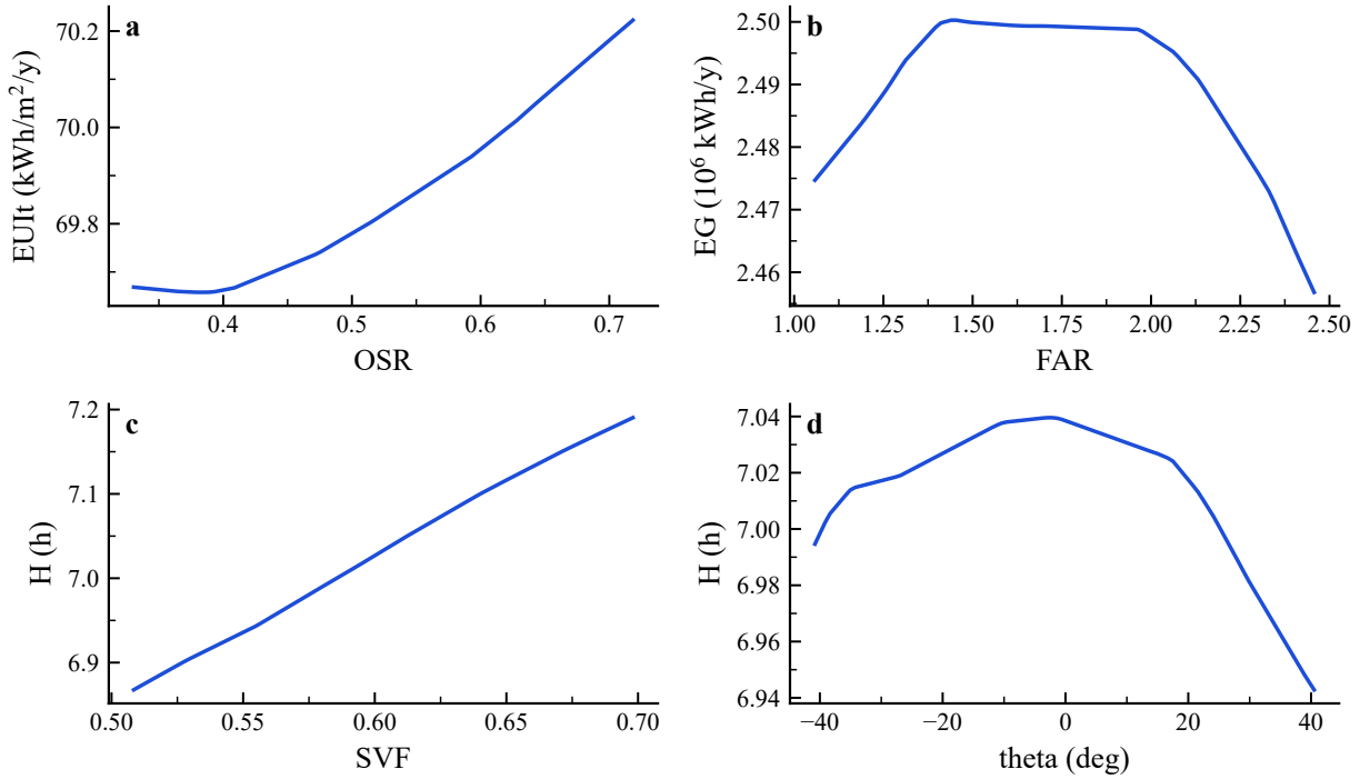
Figure B.12: Surrogate-based nonlinear response profiles for selected UMF-target pairs: (a) \text{OSR} \rightarrow \text{EUIt} , (b) \text{FAR} \rightarrow \text{EG} , (c) \text{SVF} \rightarrow \text{H} , and (d) \theta \rightarrow \text{H} .
