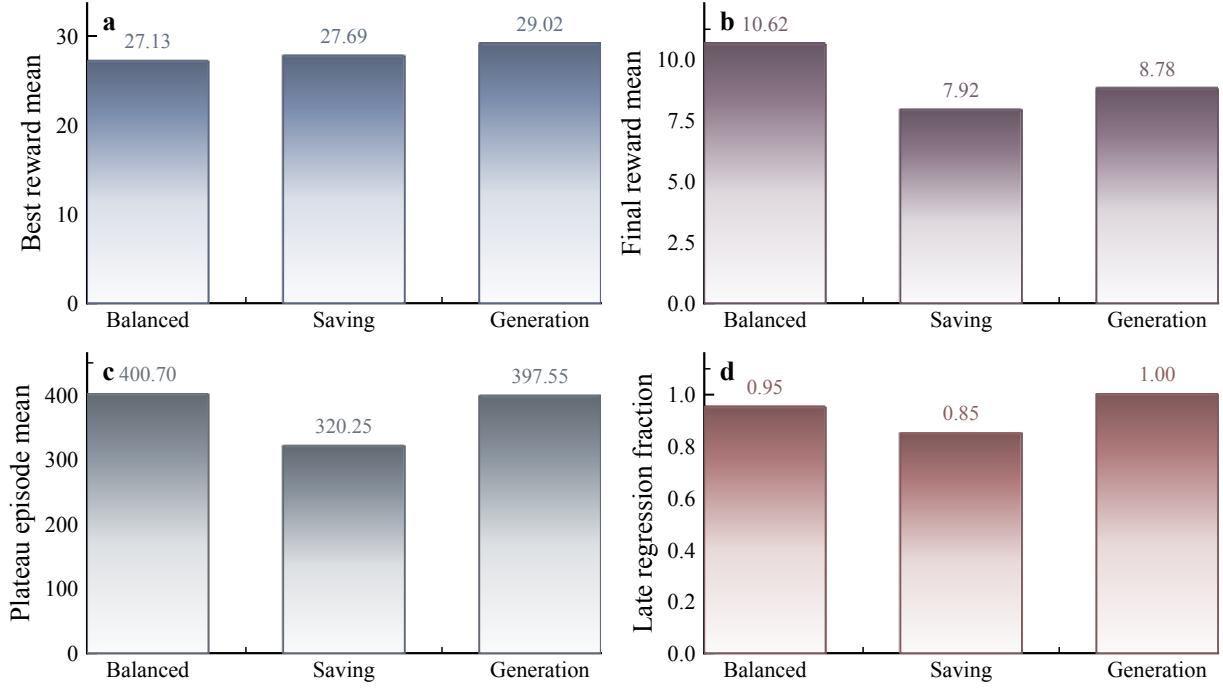
Figure 10: Seed-level convergence diagnostics on the selected 2000-sample surrogate. Panels report the mean best reward, mean final reward, mean plateau episode, and late-regression fraction across 20 seeds per DDPG scenario.
