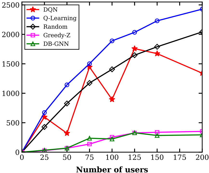
Consumed power(W)
