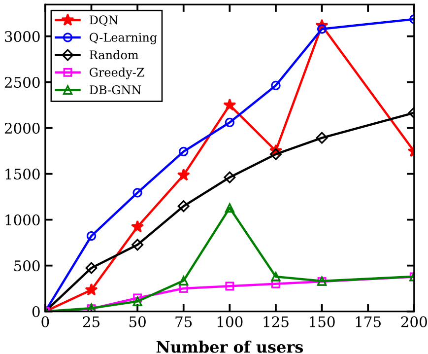
Consumed power(W)
