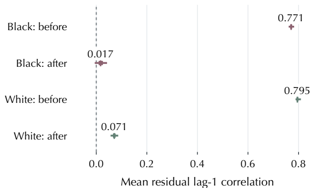
C Residual dependence Before and after the AR(1) term
