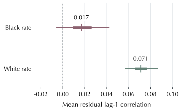
D Remaining dependence After the AR(1) term; expanded scale
