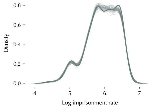
D Remaining dependence
