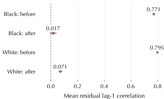
C Residual dependence
