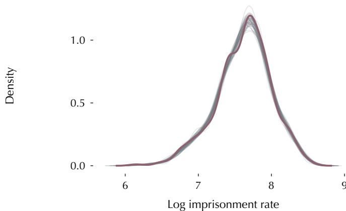
C Residual dependence
