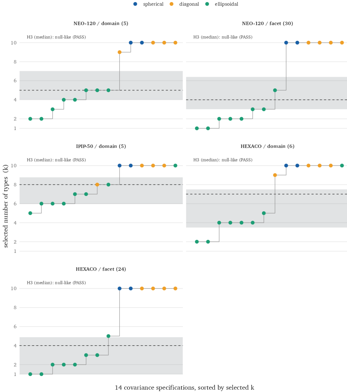
Figure 1: The BIC-selected number of mixture components (“types”) across the fourteen covariance parameterizations, on held-out data at the matched sample size. Each point is one parameterization, coloured by covariance family and sorted by selected count. The grey band marks the 95% interval of the matched-null median count; the dashed line is the real median. A real median inside the band indicates a typical count indistinguishable from data with no latent types.
