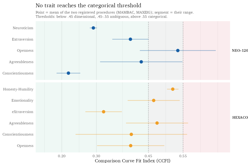
Figure 2: CCFI by trait. Each point is the mean of the two preregistered procedures, MAMBAC and MAXEIG; the segment marks their range. Values below .45 read dimensional, .45 to .55 ambiguous, above .55 categorical. No trait's registered mean reaches the categorical threshold; the full per-trait values, including the supplementary L-Mode curve, are in Table S2.
