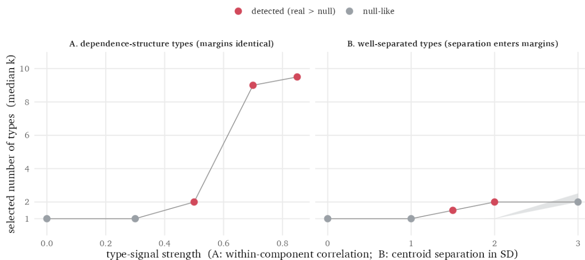
Figure 3: Positive controls on synthetic data with known structure. Grey band: the 95% interval of the matched-null median count. Points: the real median count, red where it exceeds the null. Left: types defined only by dependence (identical margins, opposite correlation orientation) are detected, increasingly so with signal strength. Right: types separated in their means are detected at moderate separation and are reproduced by the margin-preserving null only at the largest separation, where each margin is itself bimodal. Personality trait scores are unimodal, placing them in the left regime.
