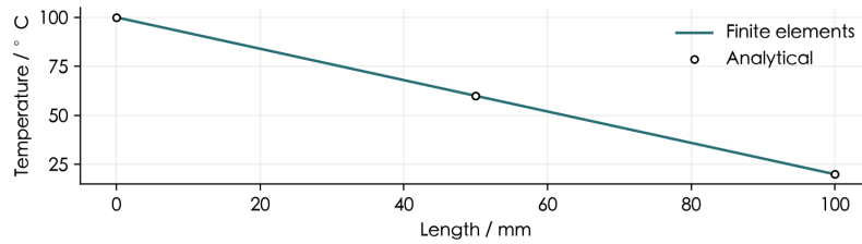
Figure 3. Temperature along the horizontal centreline.
