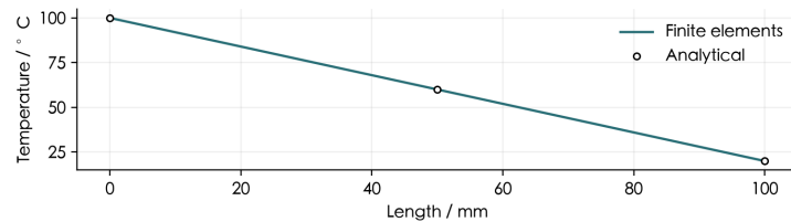
Figure 3. Temperature along the horizontal centreline.
