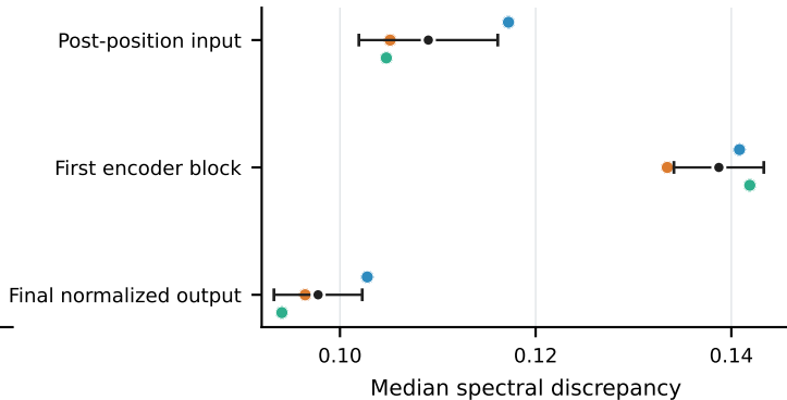
(b) Layer-wise evolution
