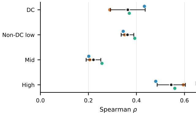
(a) Frequency-wise association
