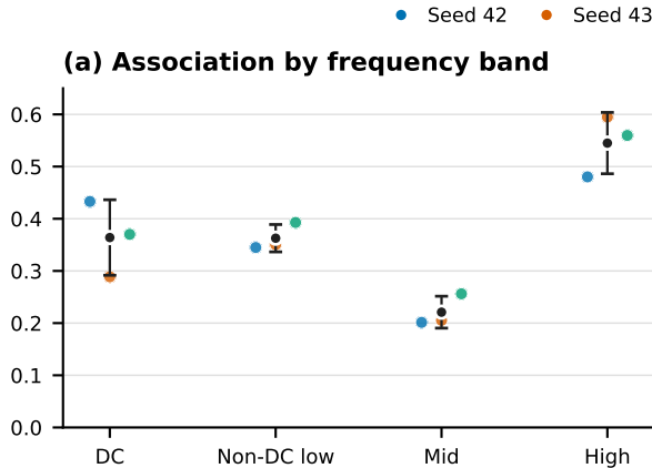
Spearman \rho with forecast MSE
