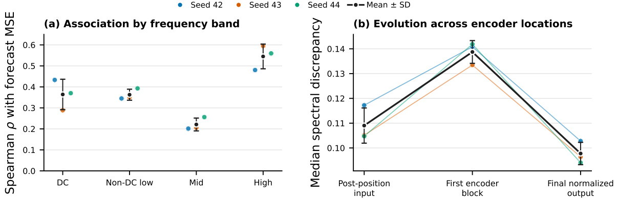
Figure 4: Frequency-wise and layer-wise summaries of the ETTh1 representation-level diagnostic across the three primary checkpoints. (a) Each colored point is the window-level Spearman association between a token-spectrum band difference and forecast disagreement for one seed; black circles and error bars are the mean and sample SD across seeds. (b) Faint colored lines connect the per-seed median token-spectrum discrepancy at the three extracted encoder locations; the black line, circles, and error bars show the mean and sample SD. These summaries describe association and representation differences in the controlled setting; they do not establish causal mediation.
