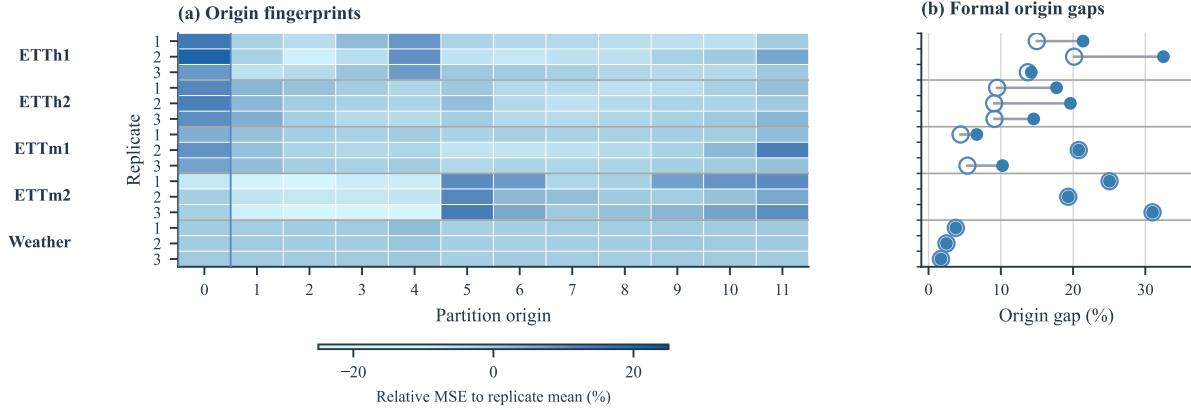
Figure 2: Origin fingerprints and formal gaps across 15 dataset–replicate profiles. Lighter-to-darker blue denotes lower-to-higher normalized relative MSE. Filled and open circles denote \Gamma_o and \Gamma_i , respectively.
