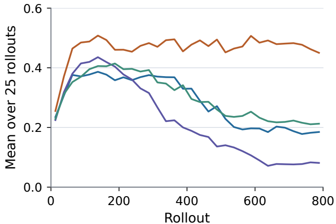
(b) Training reward
