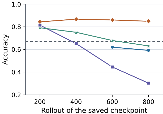
(a) MATH-500 avg@4
