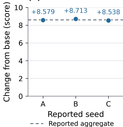
(a) HPSv3
