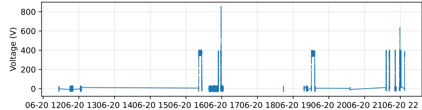
INV_DC_Bus_Voltage Over Time
