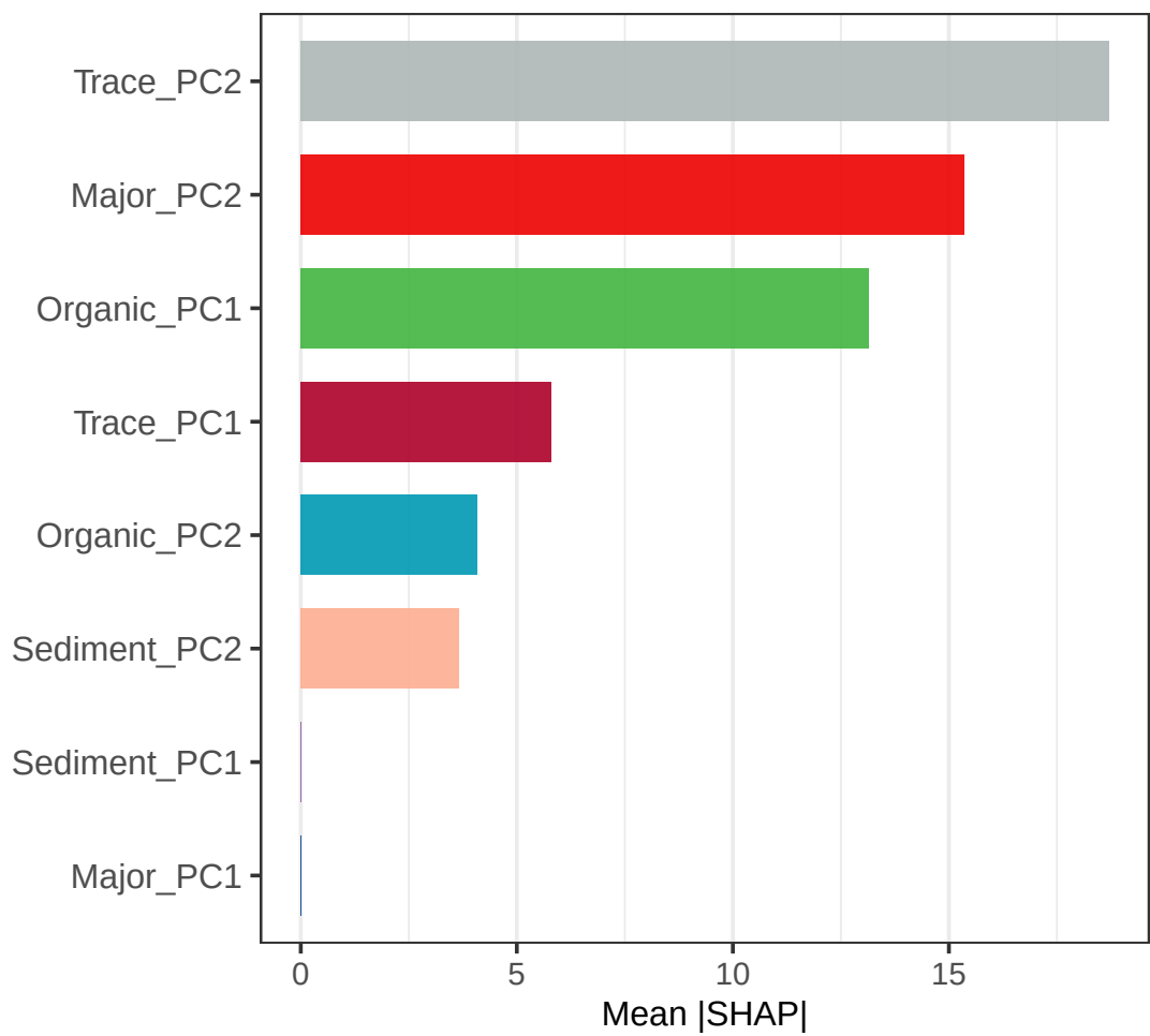
Textulariida (LightGBM)
