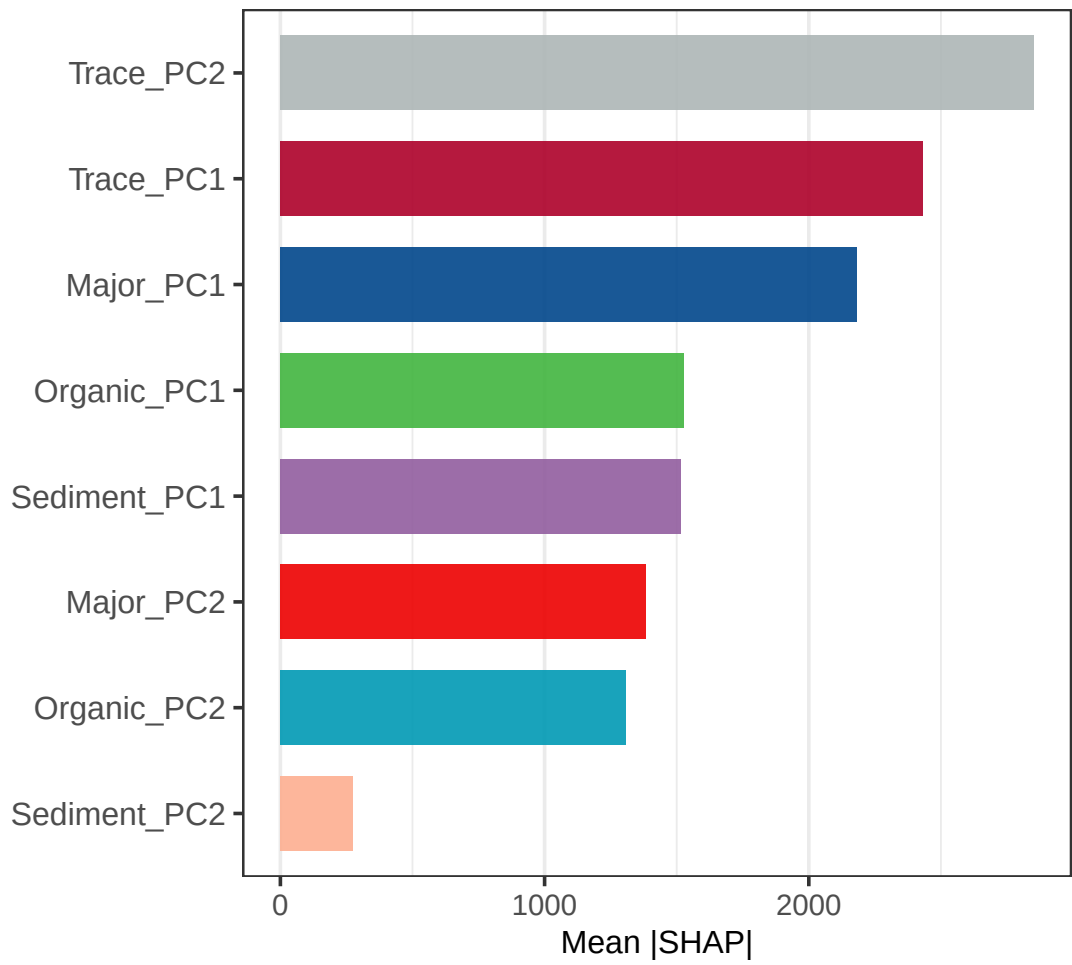
Textulariida (LightGBM)
