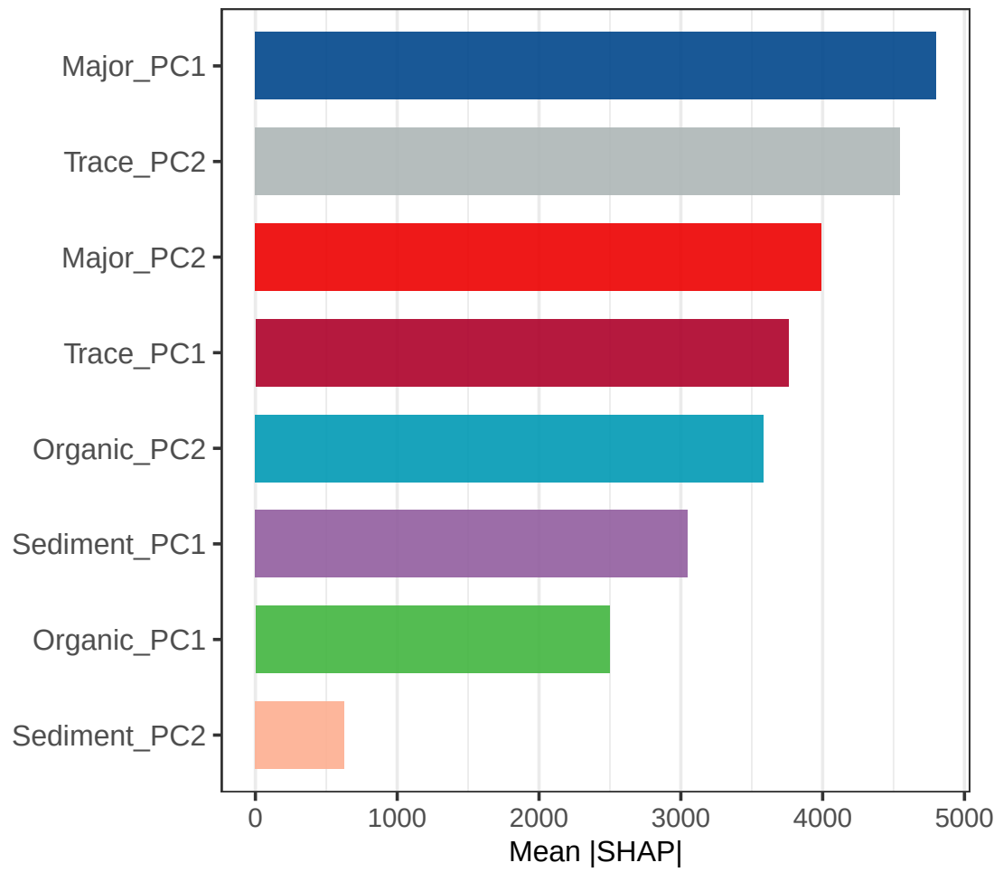
Other (RF)
