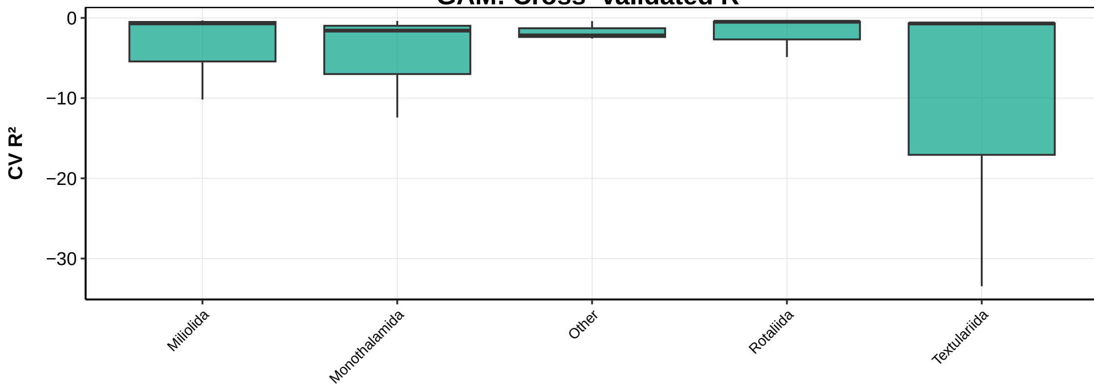
GAM: Cross-validated R 2
