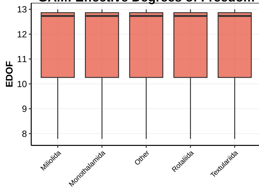
GAM: Effective Degrees of Freedom
