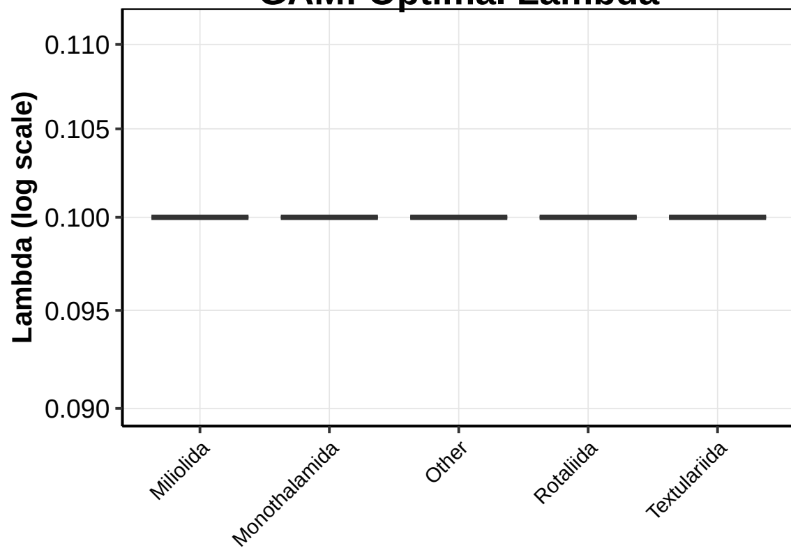
GAM: Optimal Lambda
