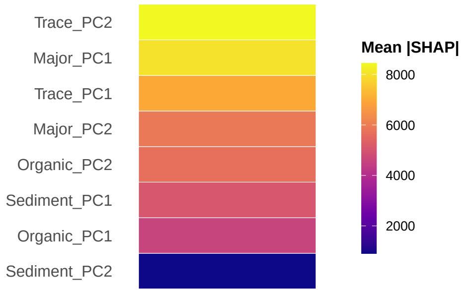
reads (RF)
