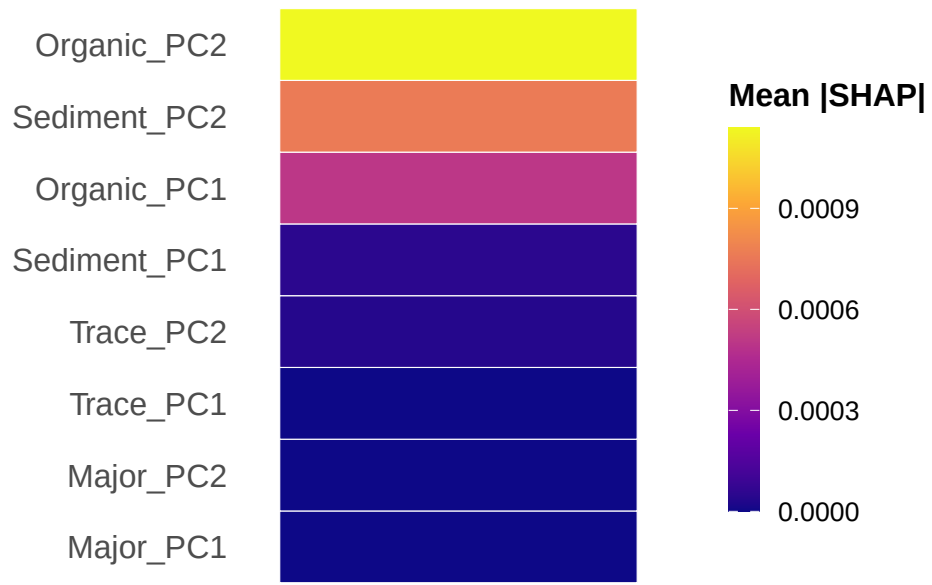
simpson (LightGBM)
