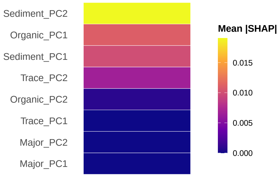
shannon (LightGBM)
