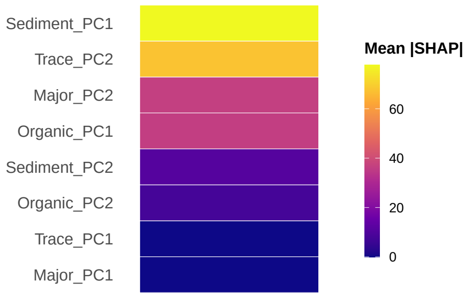
zotu (LightGBM)
