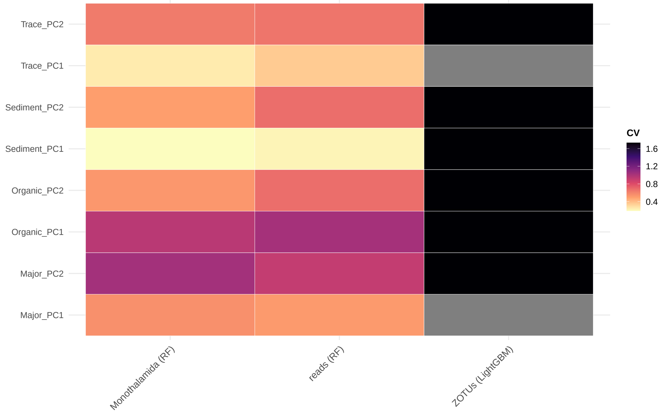
SHAP Importance Variability
