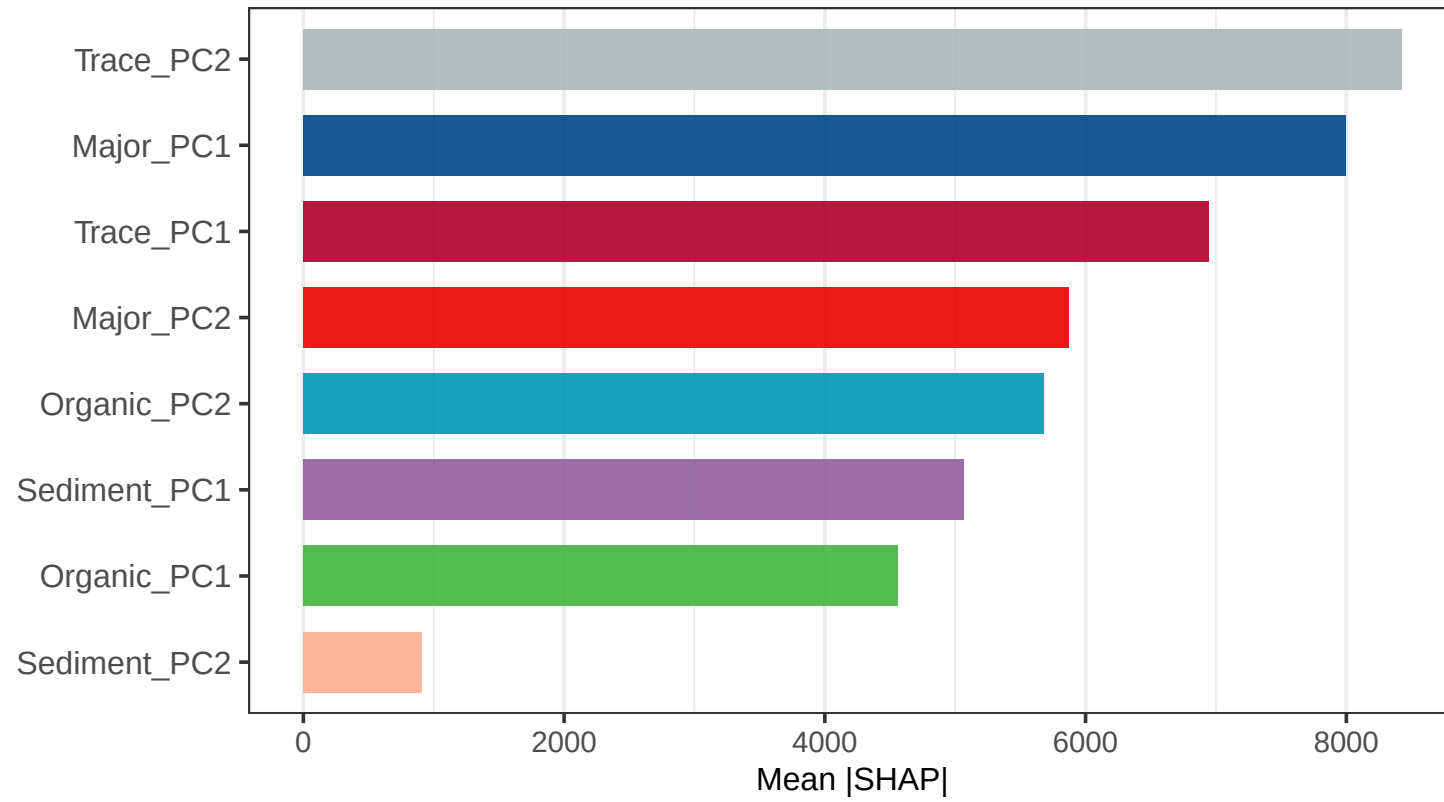
simpson (LightGBM)
