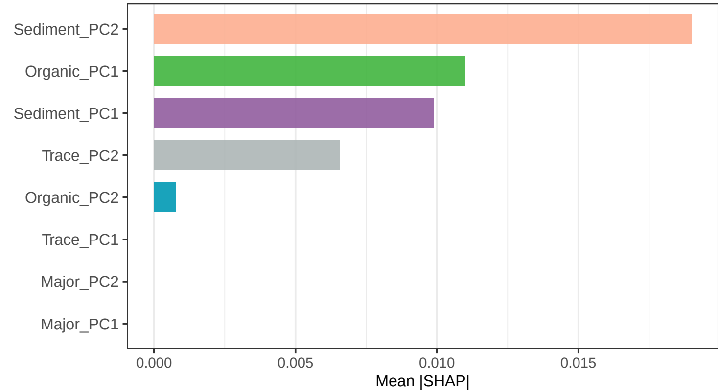
zotu (LightGBM)
