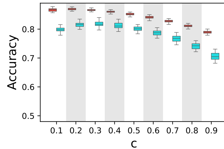
\eta(x) vs \xi(x)
