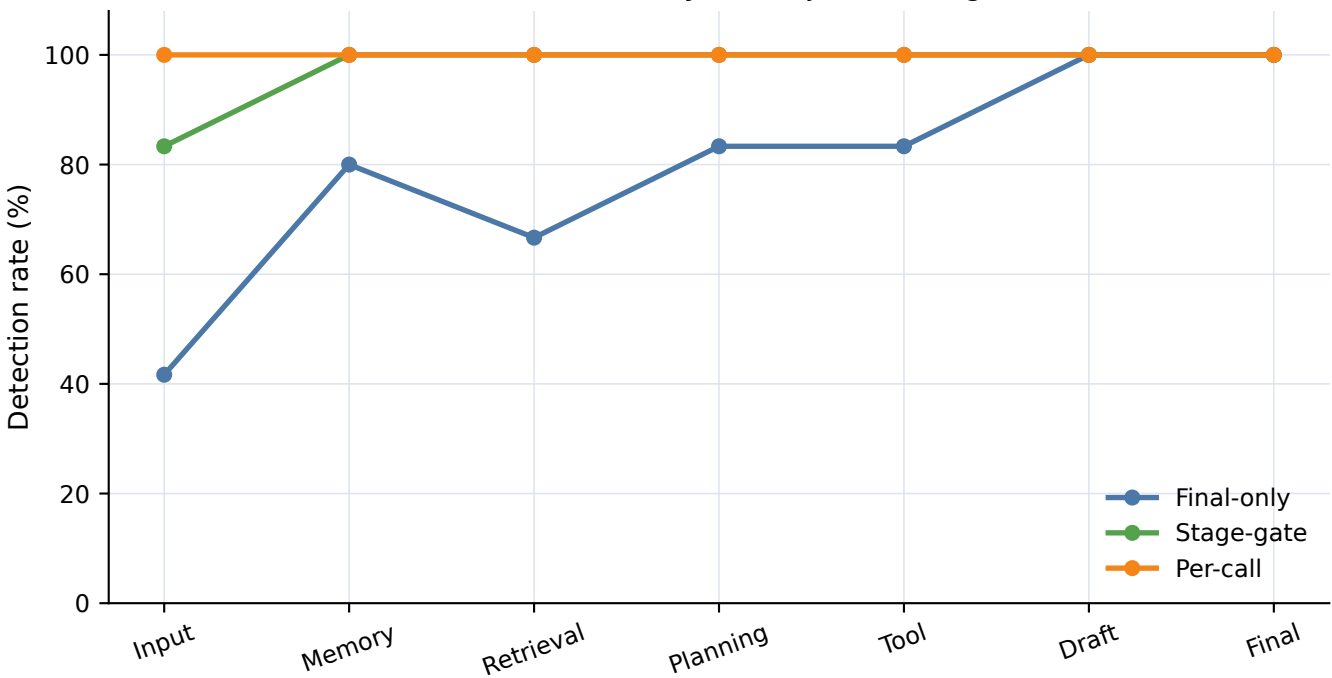
Detection Rate by Risk Injection Stage
