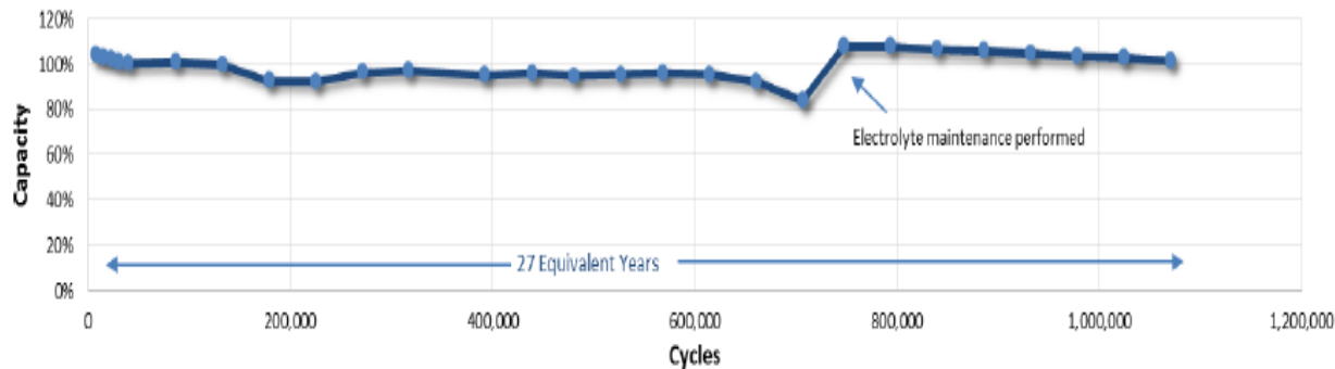
Capacity Changes Under High Frequency, High Power Cycling
