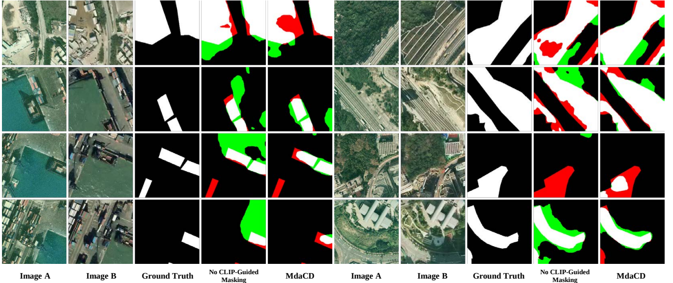
Figure 6. Qualitative ablation results of MdaCD on the SYSU-CD dataset. In the predicted masks, true positives (TP) are shown in white, true negatives (TN) in black, false positives (FP) in green, and false negatives (FN) in red. With CLIP-Guided Masking, MdaCD demonstrates improved performance in more realistic scenarios, where objects appear in both changed and unchanged regions.
