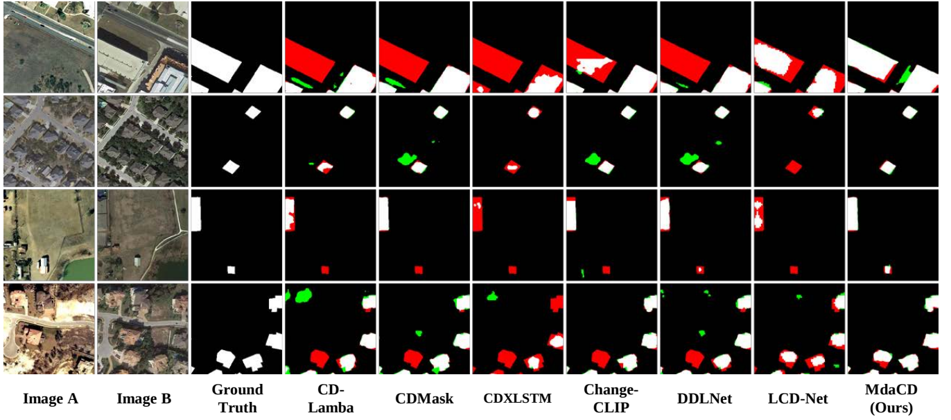
(a) Qualitative results on LEVIR-CD dataset.
