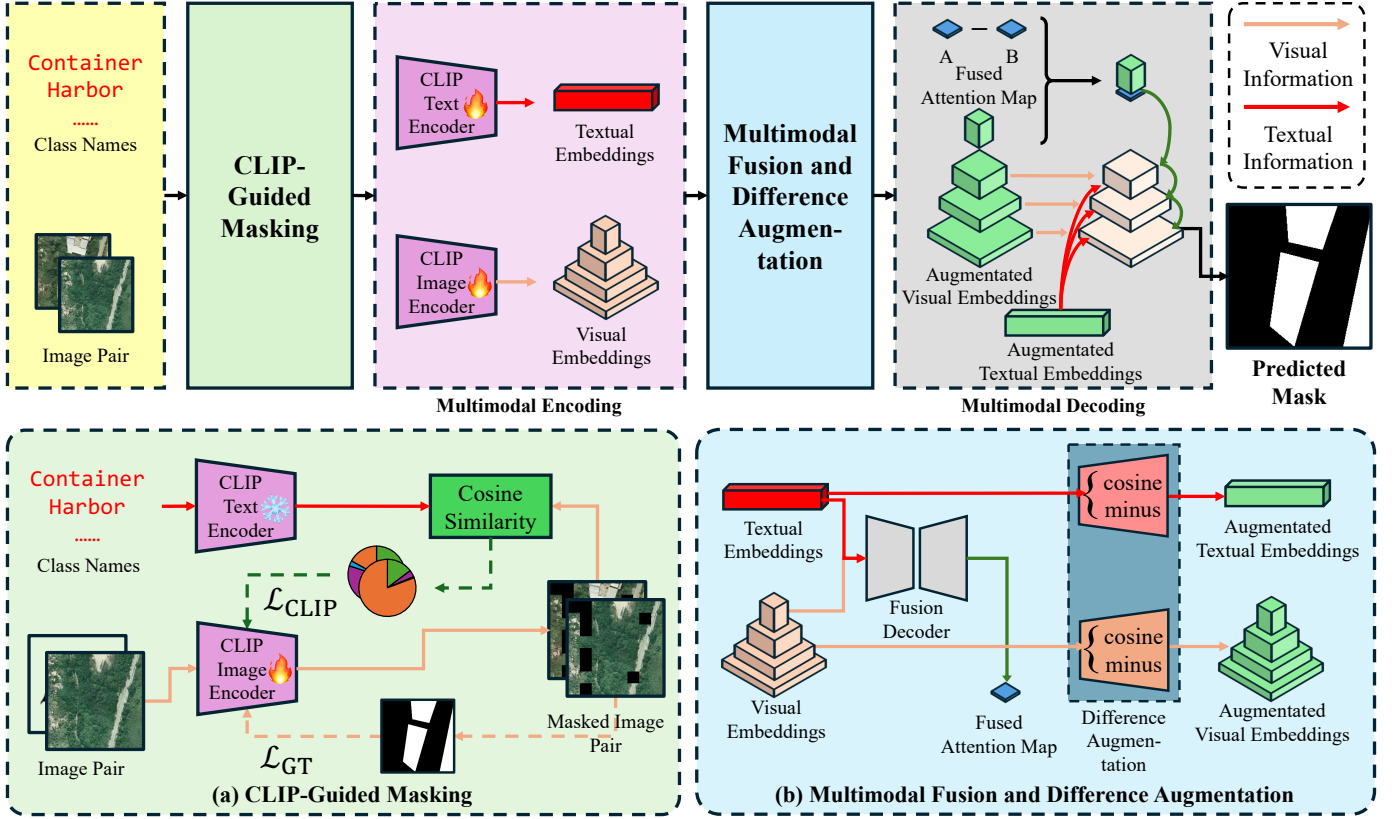
Figure 2. Overview of the proposed Multimodal Difference Augmentation Learning Change Detection Network (MdaCD). (a) Workflow of CLIP-Guided Masking process. (b) Workflow of Multimodal Fusion and Difference Augmentation process.
