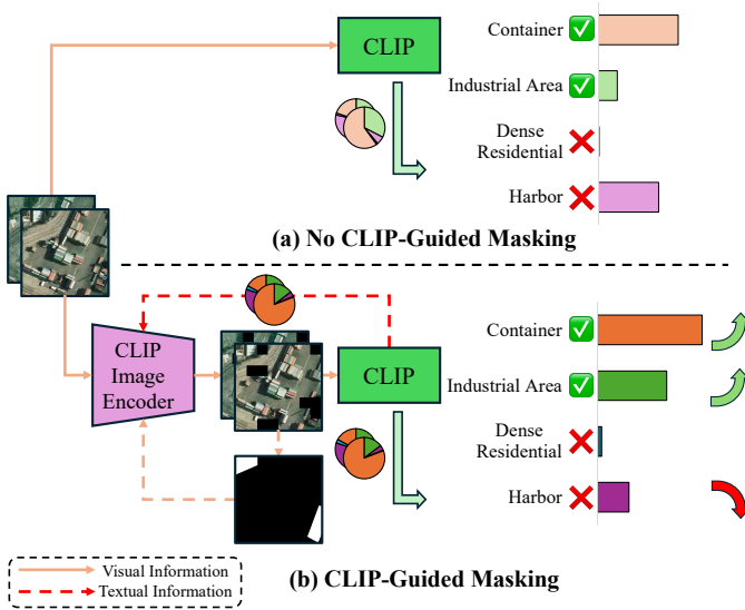
Figure 1. The textual descriptions generated by the CLIP model, along with the corresponding original and masked bi-temporal image pairs, demonstrate that changes in the images can lead to unexplainable impacts in the generated descriptions. The absolute difference between the descriptions is shown in the bar chart, while the text descriptions generated from the original and masked image pairs are represented in the first and second columns, respectively. The changed contexts are marked with a check, while the unchanged contexts are marked with a cross, indicating that the text descriptions generated from the masked image pair emphasize the changed areas more effectively.
