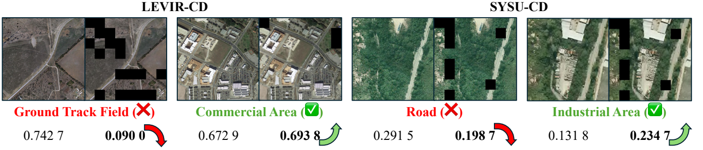
Figure 5. The text context with the highest confidence level and its corresponding confidence score (displayed below the images) for both the original and masked images from the LEVIR-CD and SYSU-CD datasets. The text context is marked in green with a check if it represents the changed context and in red with a cross if it does not. The confidence level of the masked images is highlighted in bold, indicating a stronger alignment with the actual changes.
