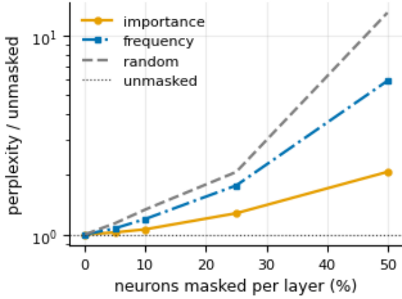
Figure 2. Qwen3.5-9B, shown separately from Figure 1. WikiText-2 perplexity divided by the unmasked baseline. Importance stays near the baseline; frequency sits between importance and random.
