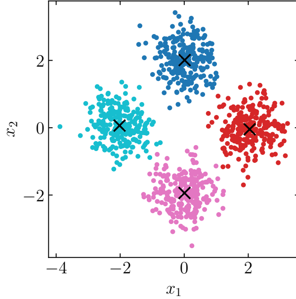
Figure 3 Results of the k -means clustering example.
