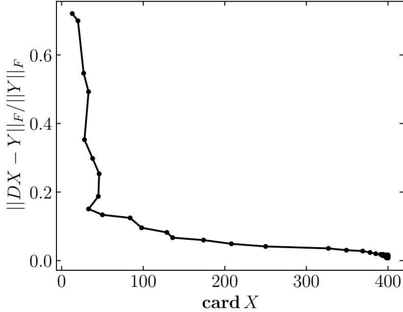
Figure 4 Trade-off curve of the sparse dictionary learning example.
