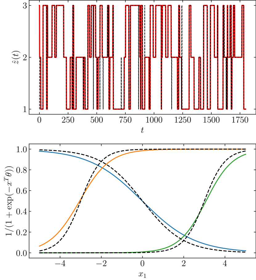
Figure 6 Results of the IO-HMM example. The ground truth state labels ( top ) and the response curve of the output probability ( bottom ) are shown in black dashed lines, whereas the corresponding estimates are shown in solid lines.
