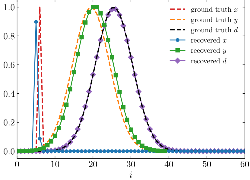
Figure 5 Results of the blind deconvolution example.
