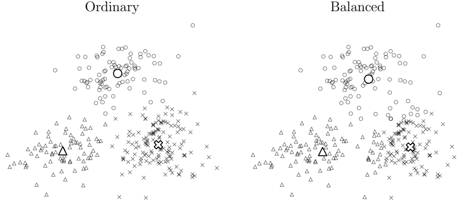
Figure 8.7 The ordinary clustering result ( left ) from the problem (8.20), and the balanced clustering result ( right ) under the constraint (8.26), on the same dataset. The final cluster representatives are shown thicker.
