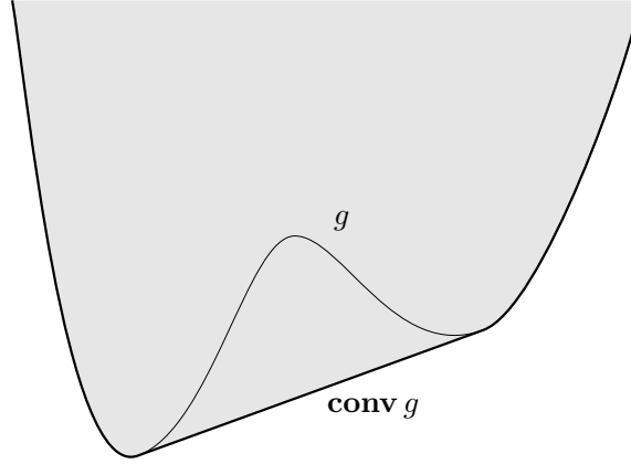
Figure 2.14 Convex envelope of the nonconvex function g is shown thicker. The epigraph of \text{conv } g is the convex hull of the epigraph of g (shown shaded).
