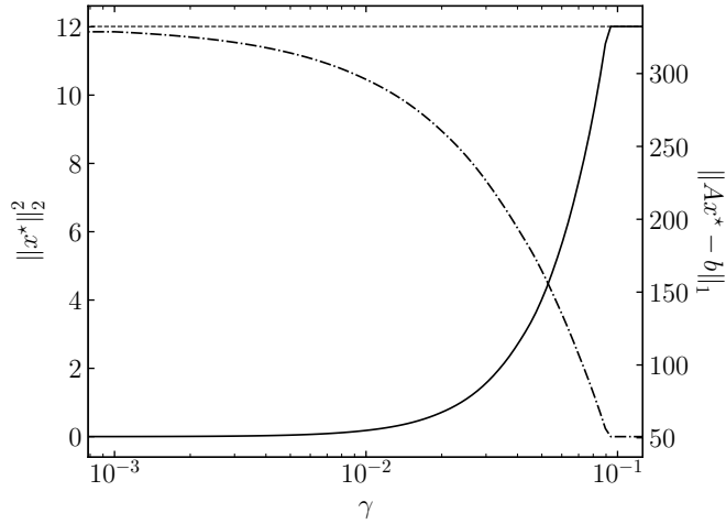
Figure 6.9 Least norm objective \|x\|_2^2 (shown solid, axis on the left) and constraint violation \|Ax - b\|_1 (shown dasheddotted, axis on the right) for the optimal point x^* of the problem (6.86) with different values of \gamma . The dashed horizontal line represents the optimal value of the least norm problem (6.85) on the largest feasible subset obtained by combinatorial search.
