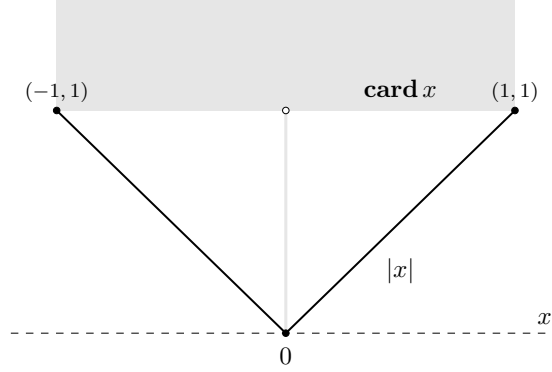
Figure 2.15 The cardinality function card x on the interval [-1, 1] . Its graph is shown as the thinner line and the dots; its epigraph is shown shaded. Its convex envelope (on the interval [-1, 1] ) is the absolute value function |x| (shown thicker).
