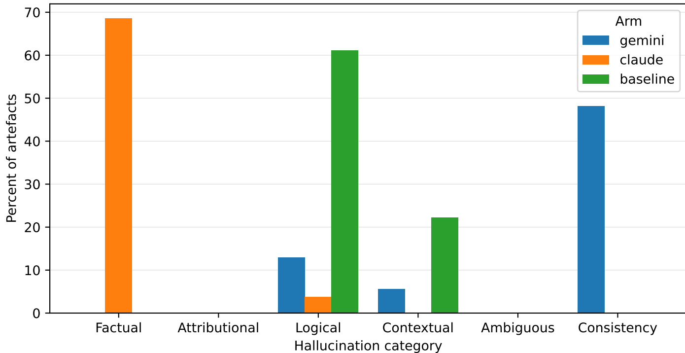
Failures rolled up to Sood's categories, by arm
