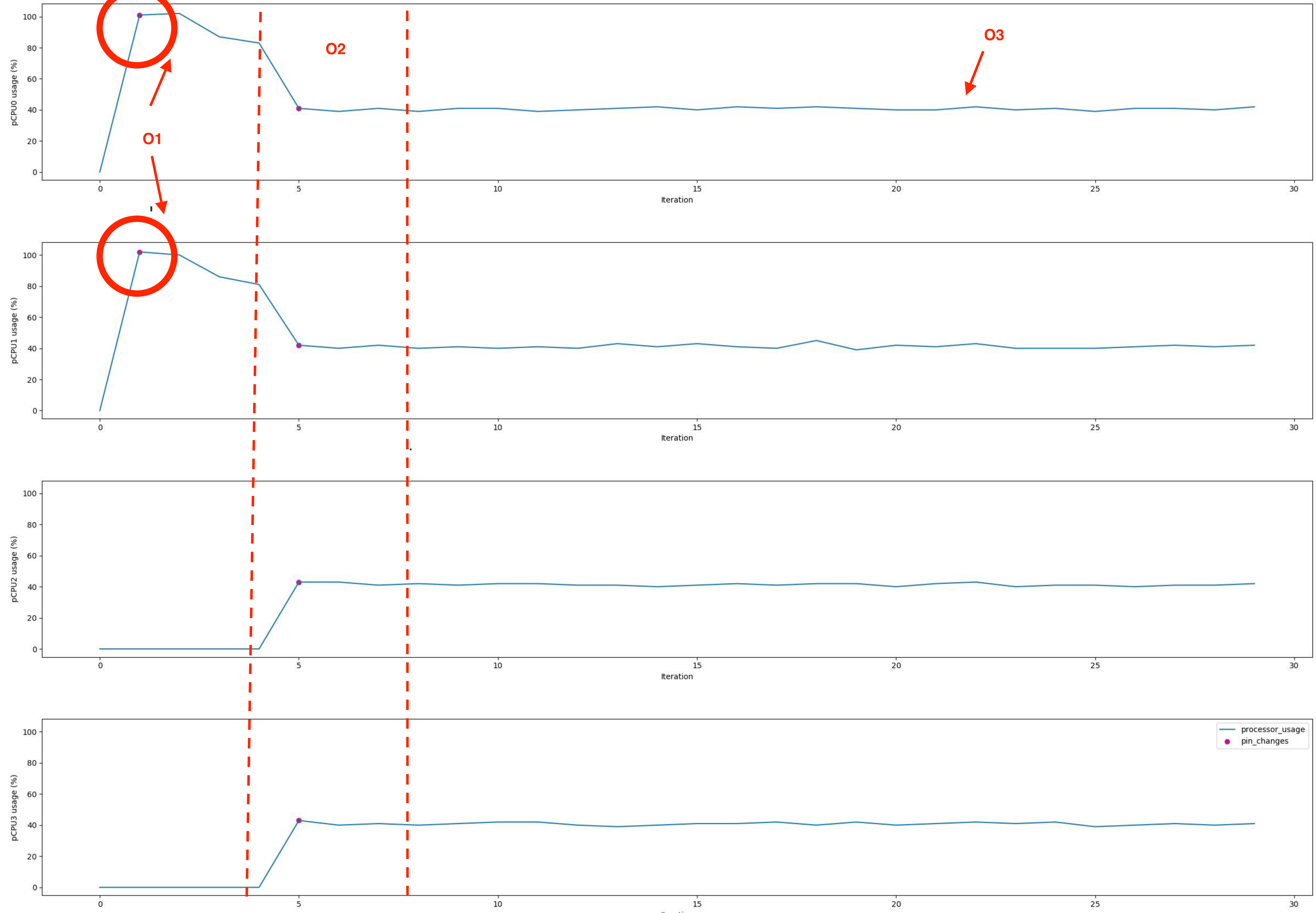
Test setup: 50% of VM's pinned to pCPU 0 and the rest to pCPU 1. Equal load on all vCPUs
