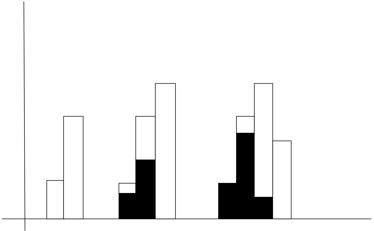
(Build-wise Graph)
