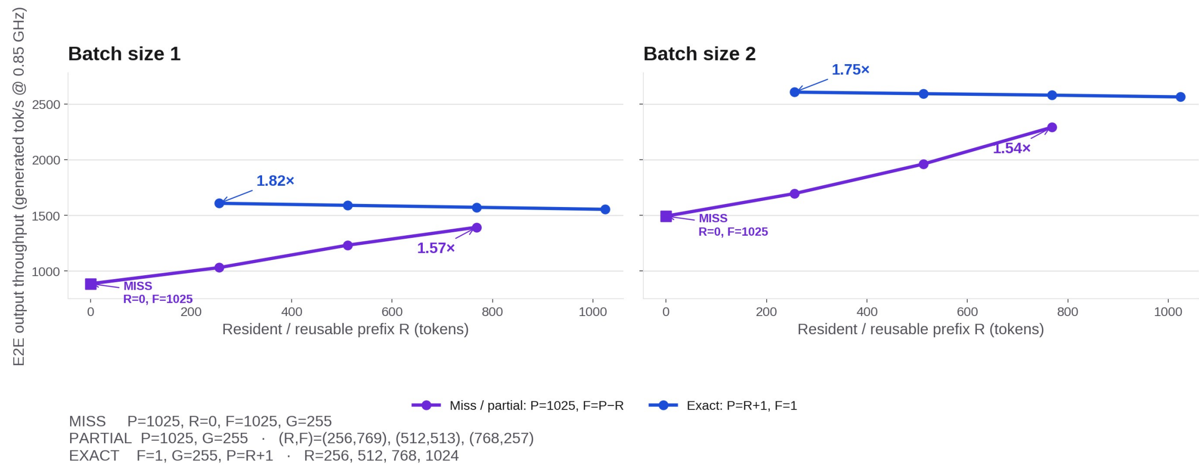
Same G=255 output budget; more resident prefix raises throughput
