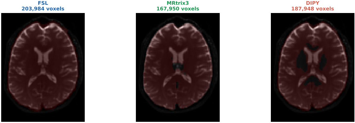
Figure 4: Brain extraction comparison on the Stanford HARDI dataset (the Sherbrooke equivalent is provided as Supplementary Figure S2). The b = 0 mean image (greyscale) with brain mask overlaid in red, produced by FSL bet (left, 203,984 voxels), MRtrix3 dwi2mask (centre, 167,950 voxels), and DIPY median_otsu (right, 187,948 voxels) from the same input volume. Dice similarity coefficients for each pair are reported in Table 3. Two differences are visible: the extent of cortical boundary coverage, and the treatment of the lateral ventricles, which DIPY median_otsu excludes while FSL bet and MRtrix3 dwi2mask retain. These reflect the distinct tissue models employed by each algorithm.
