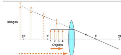
Fig. 3-20 · 6. Object between F and optical centre O → virtual, erect, magnified image on the same side (magnifying glass) [Lecture 4, p. 2]
