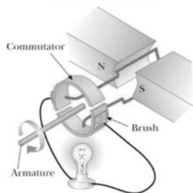
Generator DC
