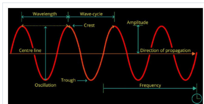
Fig. 5-1 · Anatomy of a wave — wavelength, crest, trough, amplitude, oscillation, frequency, direction of propagation [Lecture 6, p. 2]
