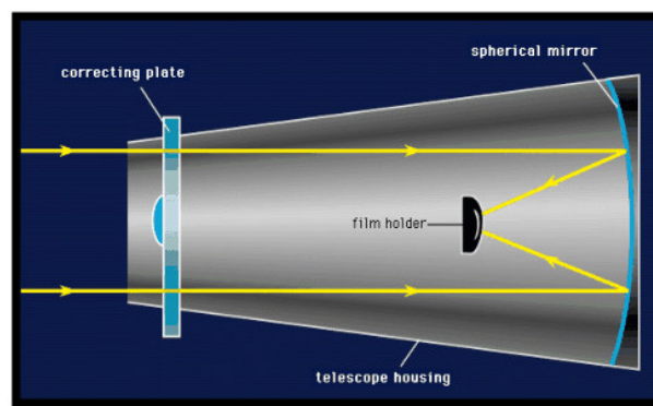
Fig. 4-16 · Reflecting telescope — correcting plate, spherical mirror, film holder [Lecture 5, p. 4]
