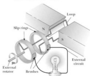
Generator AC
