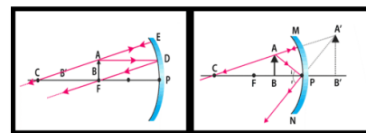
Fig. 2-19 · Object at F → image at infinity; object between P and F → virtual, erect, magnified image behind the mirror [Lecture 2, p. 4]
