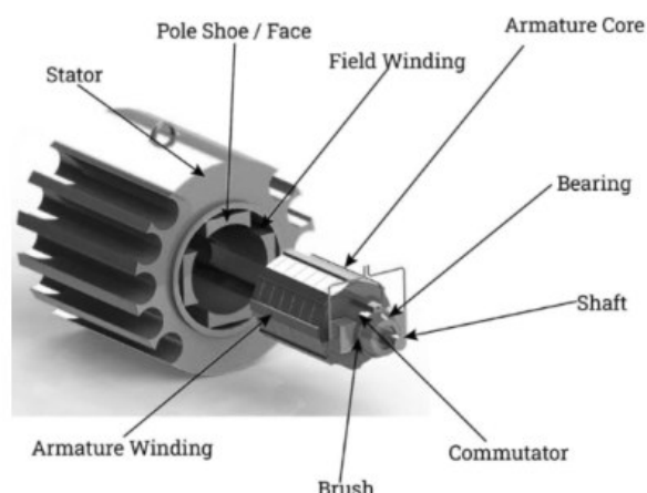
Fig. 14-8 · DC motor — stator with field winding, armature, commutator and brushes [Lecture 17, p. 3]
