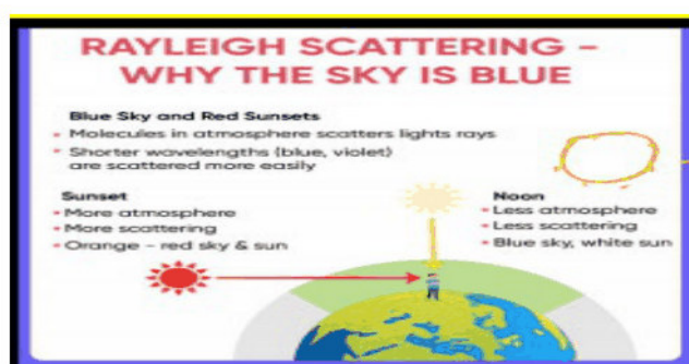
Fig. 4-7 · Rayleigh scattering — blue sky by day, red sky at sunset; more atmosphere → more scattering [Lecture 5, p. 3]
