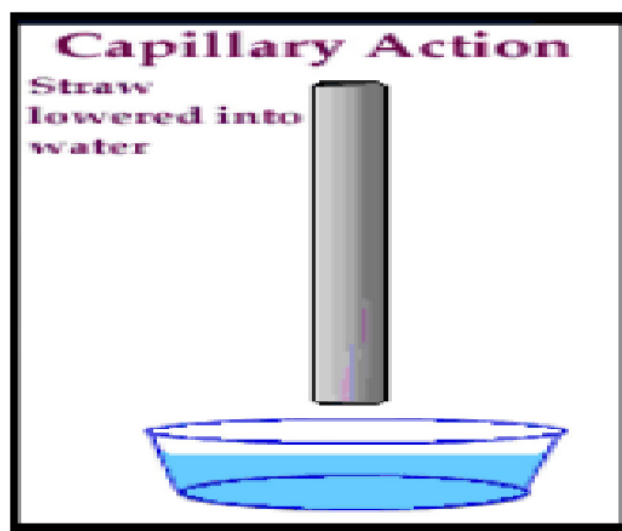
Fig. 12-9 · A straw (narrow tube) lowered into water — the liquid rises inside it [Lecture 14, p. 5]
