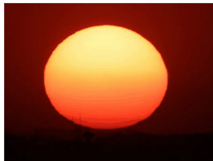
Fig. 3-7 · The setting Sun looks flattened and red [Lecture 3, p. 3]
