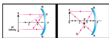
Fig. 2-17 · Object at infinity → image at F; object beyond C → between F and C [Lecture 2, p. 4]
