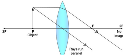
Fig. 3-19 · 5. Object at F → rays emerge parallel, image at infinity [Lecture 4, p. 2]
