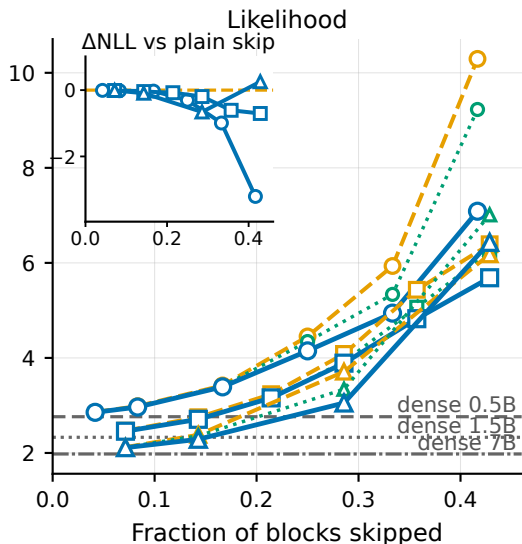
WikiText-2 NLL (lower better)
