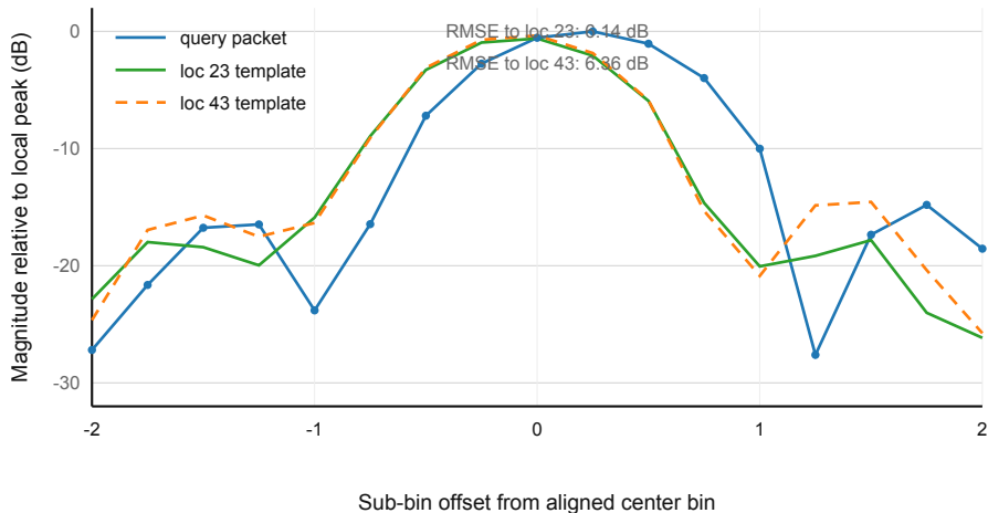
(b) q=4 preamble spectrum gives structure cue
