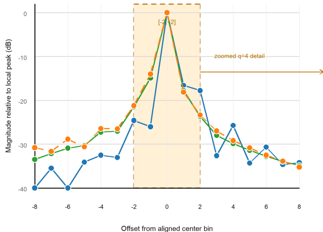
(a) Raw integer-bin spectrum, wider context
