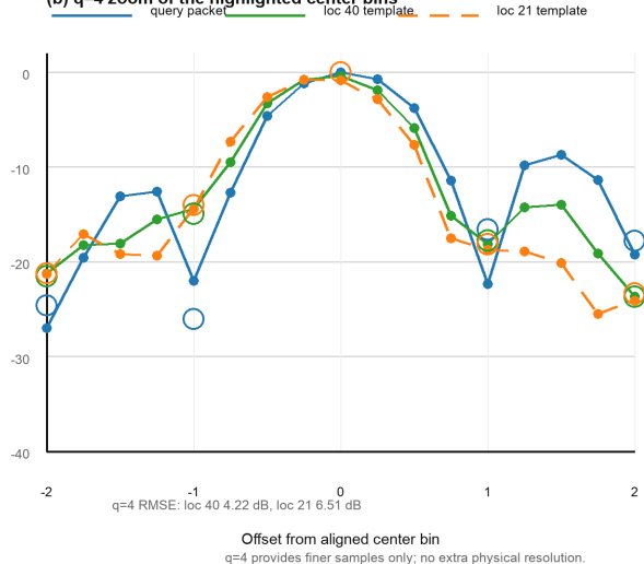
(b) q=4 zoom of the highlighted center bins
