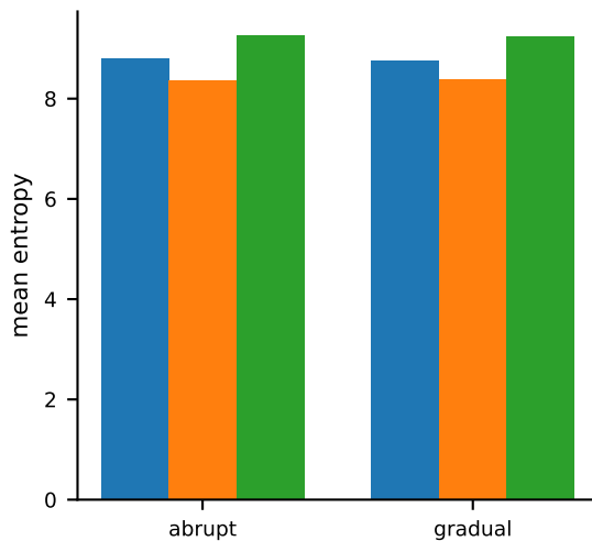
Policy entropy
