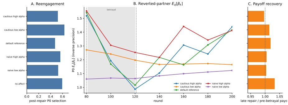
Fig. 7: Forgiveness/trust-repair diagnostic from the 20-seed profile analyses. Vertical markers indicate the transition from cooperative baseline to betrayal and then to repair/reversion. Reengagement and payoff recovery are shown alongside the reverted-partner \beta_k trajectory. Because \beta_k is inverse precision, lower \beta_k indicates higher confidence / higher policy precision; no-affect is omitted from the \beta_k trajectory panel because it has no \beta tracker. The figure shows that agents can reengage a repaired partner before rebuilding the same confidence dynamics.
