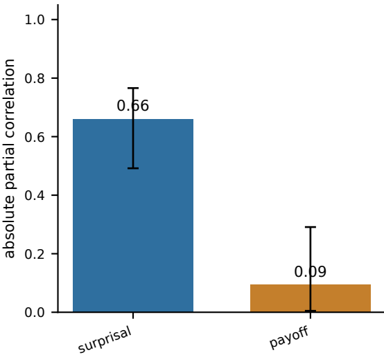
partner-local \beta
