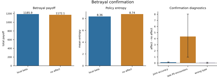
Fig. 3: Abrupt betrayal confirmation in the partner-choice regime (30 seeds). Partner-local affect lowers policy entropy relative to the no-affect control and yields a small, uncertain payoff advantage. Unlike the earlier smoke read, joint partner-type accuracy is higher under precision modulation, so the confirmation is best read as action sharpening with modest behavioral benefit rather than a payoff-accuracy tradeoff.
