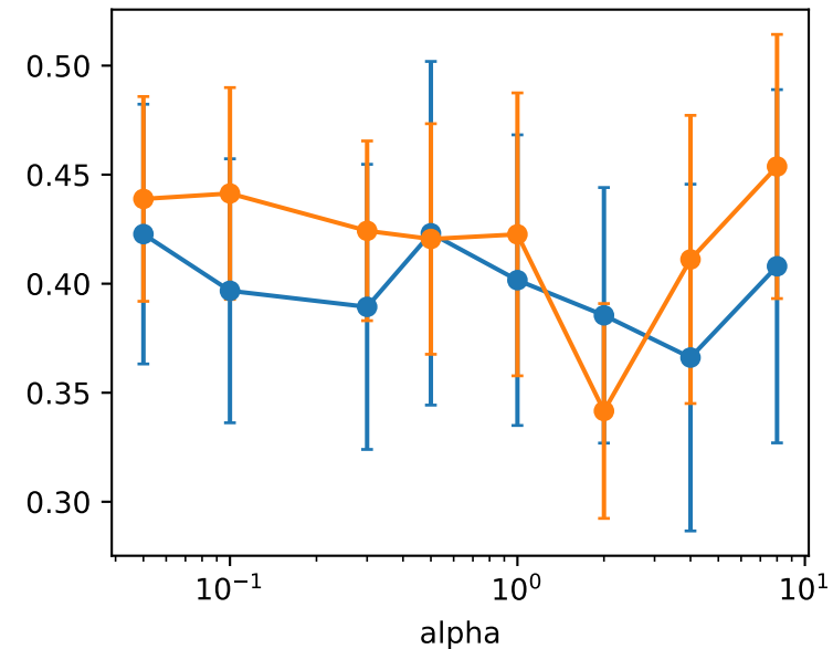
Selection Gini
