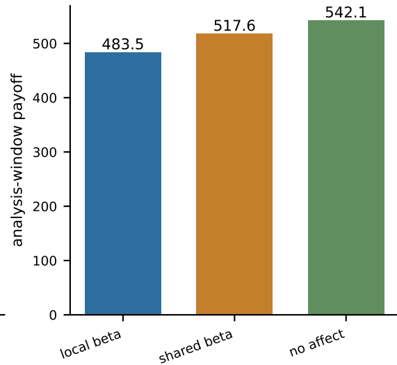
Locality-probe payoff
