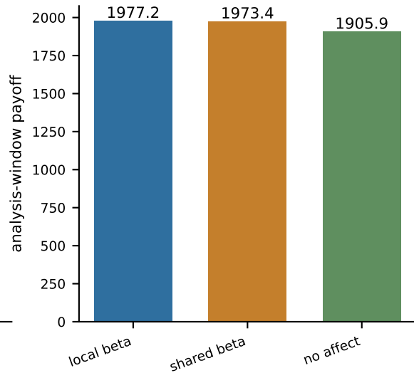
Locality-probe payoff
