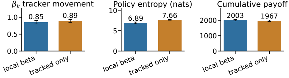
Fig. 2: Open graded regime: tracked-only and partner-local precision show comparable posterior \beta_k movement, but only partner-local precision deploys the tracker through \gamma_k and lowers policy entropy. Bars and whiskers show seed means with 95% bootstrap intervals; paired contrasts are reported in the text, and payoff is secondary.
