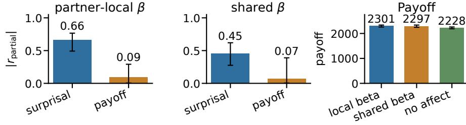
Fig. 1: Absolute active-encounter partial correlations between policy precision and surprisal/payoff, plus analysis-window payoff. Whiskers show 95% seed-cluster bootstrap intervals for correlations and seed-bootstrap intervals for payoff. Predictability is more strongly associated with partner-local than shared \beta ; because surprisal supplies the precision update, this is an intended-selectivity check.
