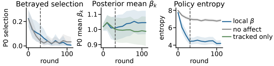
Fig. 3: Abrupt betrayal in the partner-choice regime. The dashed line marks partner 0’s round-31 stance switch; bands show 95% seed-bootstrap intervals. Partner-local precision maintains lower policy entropy after the switch, while tracked-only \beta_k dynamics persist without the same deployment effect; selection shows redistributed engagement.
