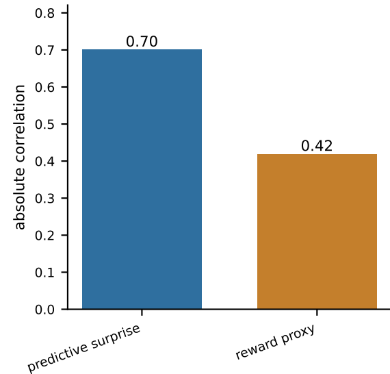
Precision correlations
