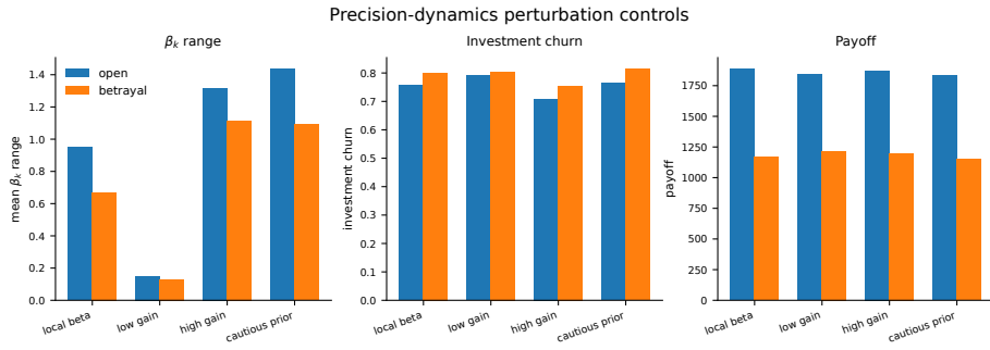
Fig. 4: Perturbation controls in the graded decision regime (Table 7).
