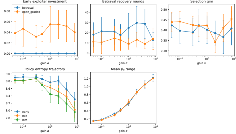
Fig. 5: Precision-gain sweep across open graded and betrayal environments. Higher \alpha expands \beta_k range, while engagement, recovery, entropy, and payoff readouts vary non-monotonically. Precision gain therefore controls confidence-reactivity amplitude rather than mapping directly to reward.
