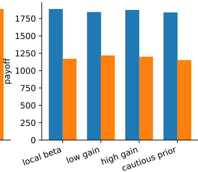
Total payoff
