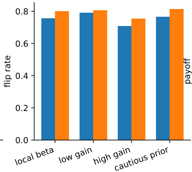
Action churn
