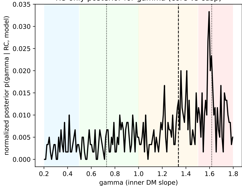
RC-only posterior for gamma (core vs cusp)
