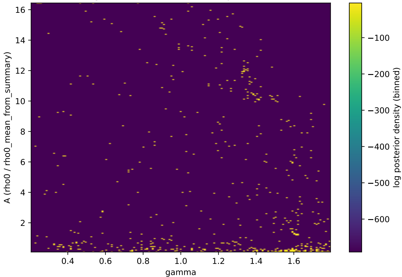
RC: (gamma, A) from NUTS samples (binned)
