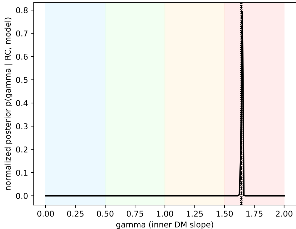
RC-only posterior for gamma (core vs cusp)
