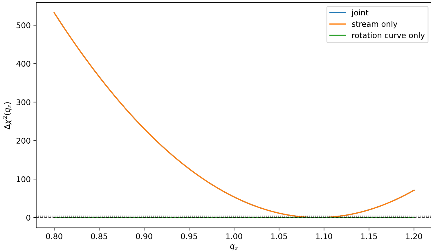
Joint q_z with physical Beordo2024 rotation curve (acceleration-based)
